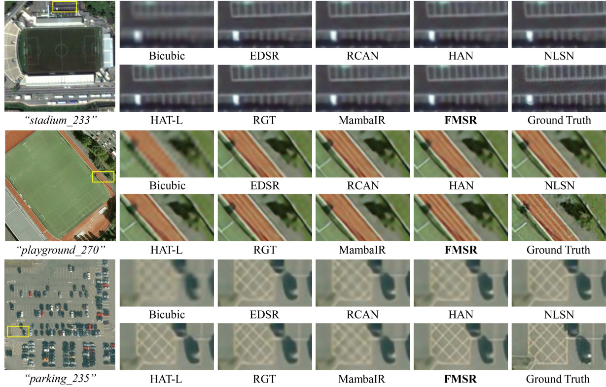
Fig. 11. Visual comparisons of our FMSR with CNN-, Transformer-, and Mamba-based methods on AID [62] with scale \times 4 . Zoom in for better observation.
