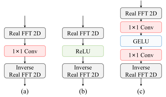
Fig. 4. Three variants of Frequency Selection Module (FSM). Here, we adopt 2D Fast Fourier Transformation (FFT) for frequency learning.
