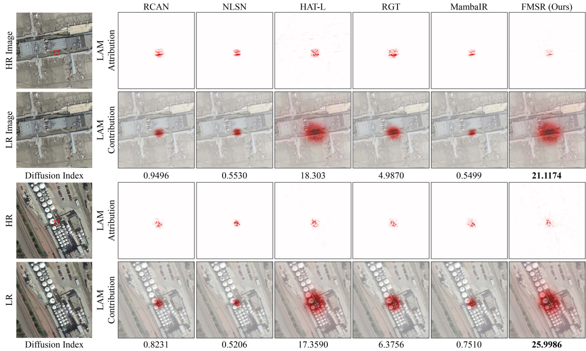
Fig. 10. The visualization of Local Attribution Maps (LAM) [67]. A wider range of LAM illustrates more pixels are involved in reconstruction. A higher diffusion index demonstrates better global activation capability.
