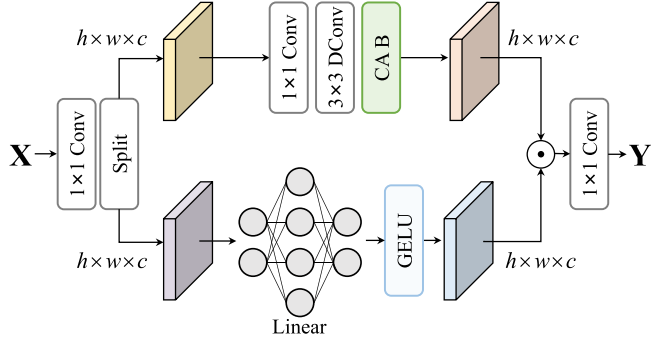
Fig. 3. The proposed Hybrid Gate Module (HGM) conceptual illustration. The input feature X is split in the channel dimension and fed through a Channel Attention Block (CAB) and a pixel-wise linear projection layer, respectively. After a Hadamard product operation, a 1 \times 1 convolution generates the output tensor Y .
