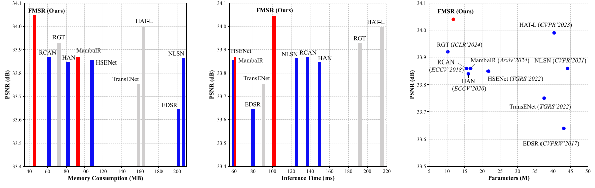
Fig. 9. Ablation studies of memory consumption, inference times, parameters, and PSNR performance on DOTA [63]. Note that the inference times are calculated on 100 images.
