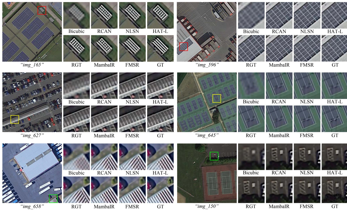
Fig. 12. Visual comparisons of our FMSR with CNN-, Transformer-, and Mamba-based methods on DOTA [63] with scale \times 4 . Zoom in for better observation.
