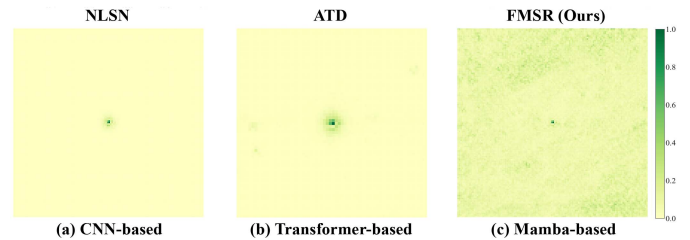
Fig. 1. The Effective Receptive Field (ERF) [21] comparison for (a) CNN-based method NLSN [22], (b) Transformer-based model ATD [23], and the proposed Mamba-based network FMSR. A wider distribution of dark areas demonstrates larger ERF. Our FMSR effectively obtains the largest ERF, indicating favorable global exploration capability.
