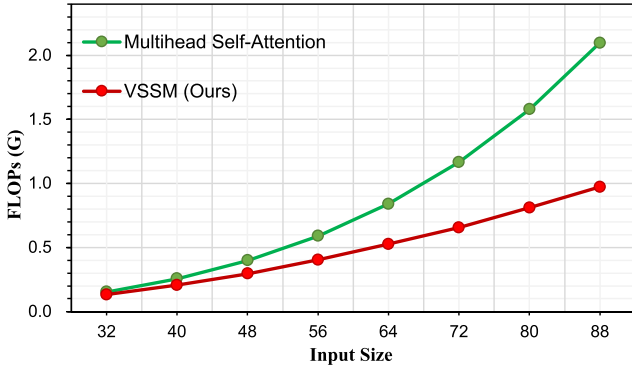
Fig. 8. Computational complexity comparison with inputs of different resolutions. We adopt the standard Multihead Self-Attention [1] as the baseline. Initially, we adjust the model to ensure that the consumption of parameters and FLOPs is roughly equivalent. Subsequently, we increase the input resolution from 32 \times 32 to 88 \times 88 .
