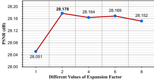
Fig. 7. Ablation studies on the effect of different expansion factors \lambda .
