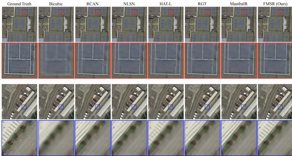
Fig. 13. Visual comparisons of our FMSR with CNN-, Transformer-, and Mamba-based methods on DIOR [65] with scale \times 4 . Zoom in for better observation.
