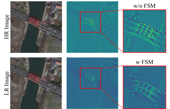
Fig. 6. Visualization of the feature maps. The proposed Frequency Selection Module (FSM) yields sharp and clear details for reconstruction.
